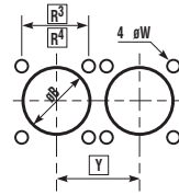
Square Flange receptacle rear panel mounting
